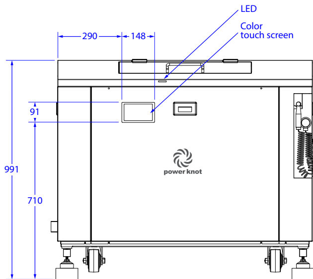
Front
